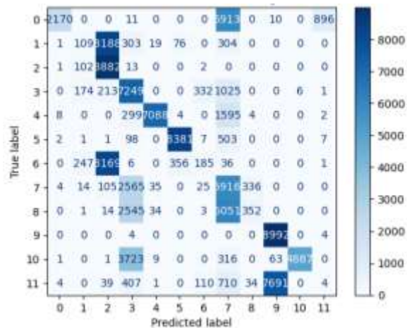
Gambar 8. Confusion Matrix Model Naive Bayes
